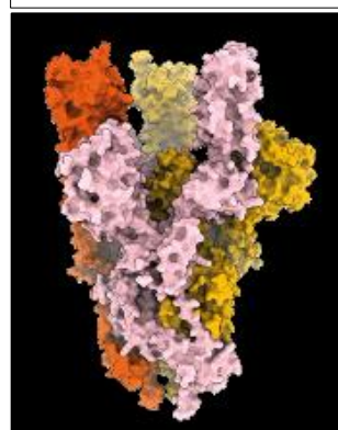
Figure 1: Scheme, a- of virtual energy levels of a molecular system undergoing successive reactions, b-global structure of Covid-19 virus [2].
