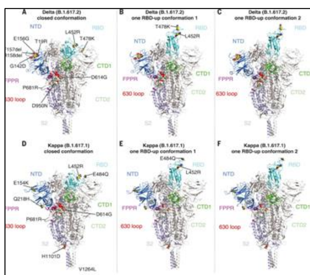
Figure 2: Scheme of some discovered mutations of Covid-19 virus. [3]
