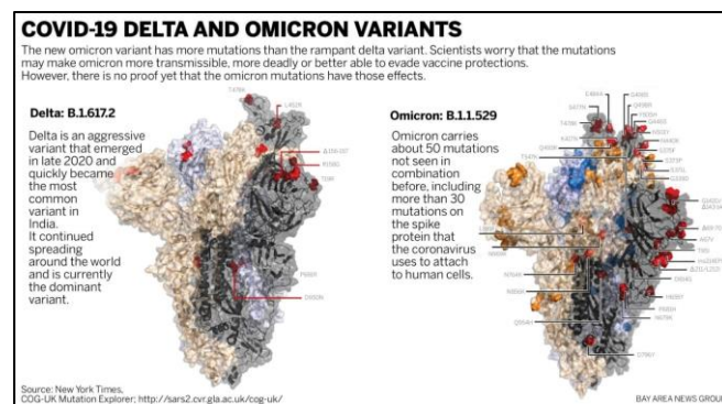
Figure 3: Covid-19 Delta & Omicron variants. [5]
